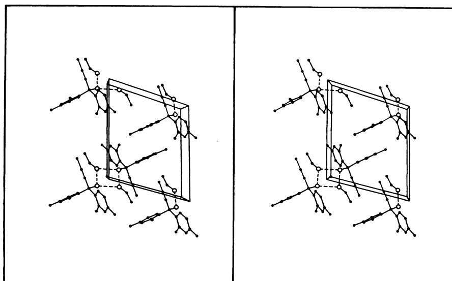
Fig. 5. Stereo view of the crystal structure of the 1:1 adduct (II) of 1,1-bis(2,4-dimethylphenyl)-2-butyne-1-ol ( 3c ) with ethanol. The origin of the unit cell lies at the lower left corner, with a pointing towards the reader, b slantwise from left to right, and c upwards. The disordered methyl group of the ethanol molecule is shown in one of its two half-populated sites, and hydrogen bonds are represented by broken lines.
