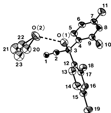
Fig. 1. Perspective view and atom labelling of the asymmetric unit in I. Both orientations of the disordered ethyl group are shown, and the broken line represents an O(1)···O(2) hydrogen bond.
