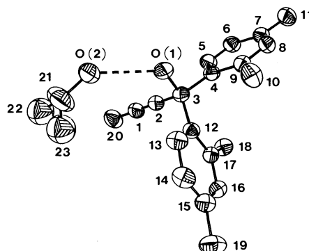
Fig. 2. Perspective view and atom labelling of the two molecular components in II. Both orientations of the disordered methyl group are shown, and the O(1)···O(2) hydrogen bond is represented by a broken line.
