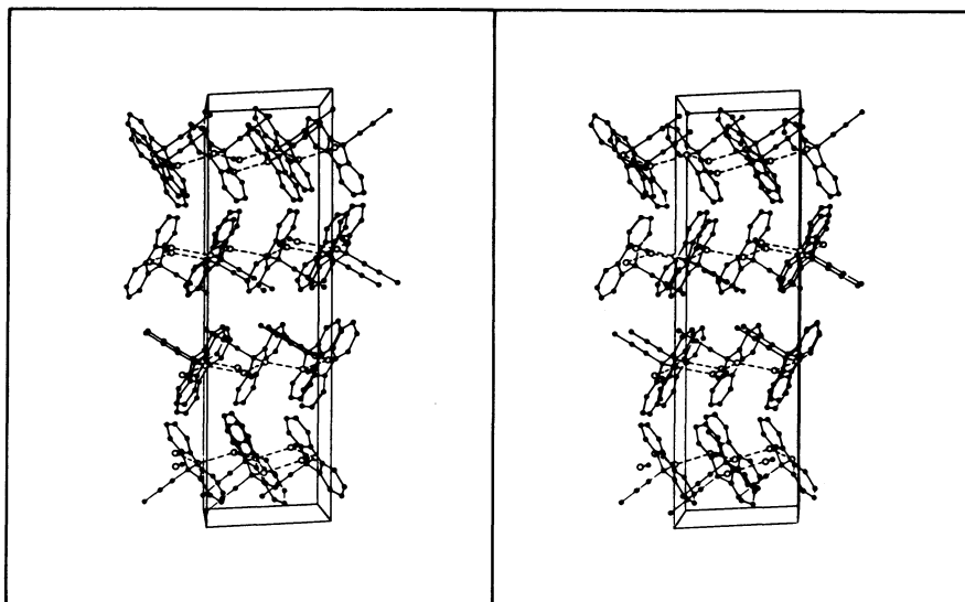
Fig 6. Stereo view of the crystal structure of the 1:1 adduct (III) of 9-hydroxy-9-(1-propynyl)fluorene ( 4 ) with methanol. The origin of the unit cell lies at the upper right corner, with a pointing from left to right, b towards the reader, and c downwards. Hydrogen bonds are represented by broken lines.
