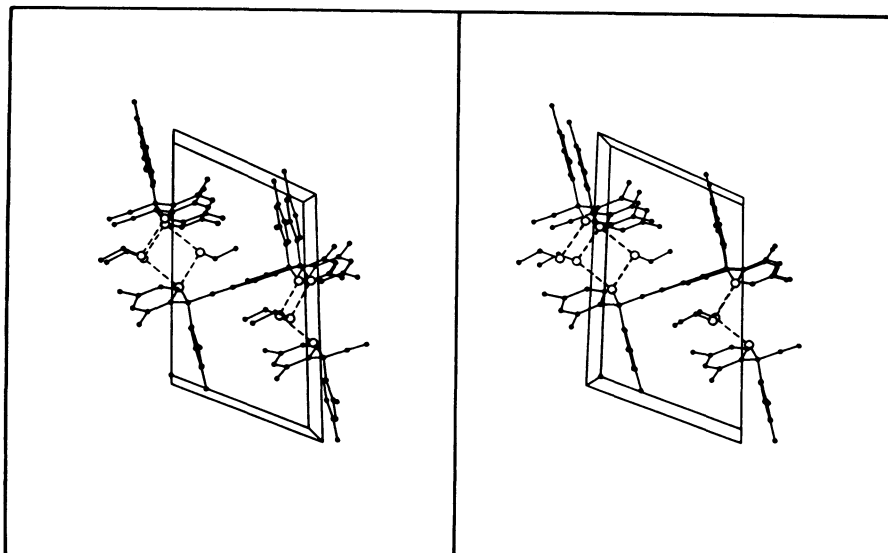
Fig. 4. Stereo view of the crystal structure of the 1:2 adduct (I) of 1,1,6,6-tetrakis(2,4-dimethylphenyl)-2,4-hexadiyne-1,6-diol ( 2b ) with ethanol. The origin of the unit cell lies at the lower left corner, with a pointing towards the reader, b slantwise from left to right, and c upwards. The disordered ethyl group is shown in one of its two orientations, and hydrogen bonds are represented by broken lines.
