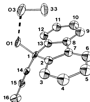
Fig. 3. Perspective view and atom labelling of one set (Type A) of molecular components in III, the O(1)···O(3) hydrogen bond being shown as a broken line. Atom labels for the other fluorene and methanol molecules (Type B) in the asymmetric unit are derived by incrementing the numbering of the corresponding oxygen and methanol carbon atoms by 1, and that of the remaining carbon atoms by 16.
